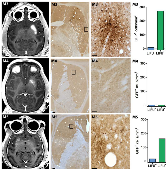
Fig. 5. Delivery of modified AAV9 vectors after large-volume BBB openings in the putamen of normal and parkinsonian NHPs. Representative images of distributions of Gd extravasation ( first column ) and GFP + cells (low and higher magnifications in second and third columns , respectively) in the putamen of M3, M4, and parkinsonian monkey M5. Note that the distribution areas of GFP + cells overlap the regions of Gd extravasation observed immediately after sonication, except for monkey M4 which had NABs against AAV and, therefore, displayed no GFP expression. Fourth column shows the number of GFP + cells in the BBB-opened regions (LIFU + ) and their contralateral non-opened regions (LIFU - ) for each monkey. Scale bars, 1 mm (for low magnifications in second column) and 50 \mu m (for higher magnifications in third column).
