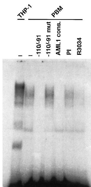
FIG. 5. Nuclear extracts from peripheral blood monocytes contain PEBP2/CBF factors that bind to the CD36 promoter PEBP2/CBF site. Radiolabeled double-stranded CD36 promoter -110/-91 oligonucleotide was incubated with nuclear extracts from THP-1 cells and from peripheral blood monocytes. Prior to adding the radiolabeled oligonucleotide, nuclear extracts from monocytes were incubated with a 50-fold molar excess of the cold double-stranded oligonucleotides -110/-91, -110/-91 mut, and AML1 cons. (see Fig. 4 legend for details) or with rabbit preimmune sera (PI) or AML1-specific antisera R3034. -, no inhibitor added.
