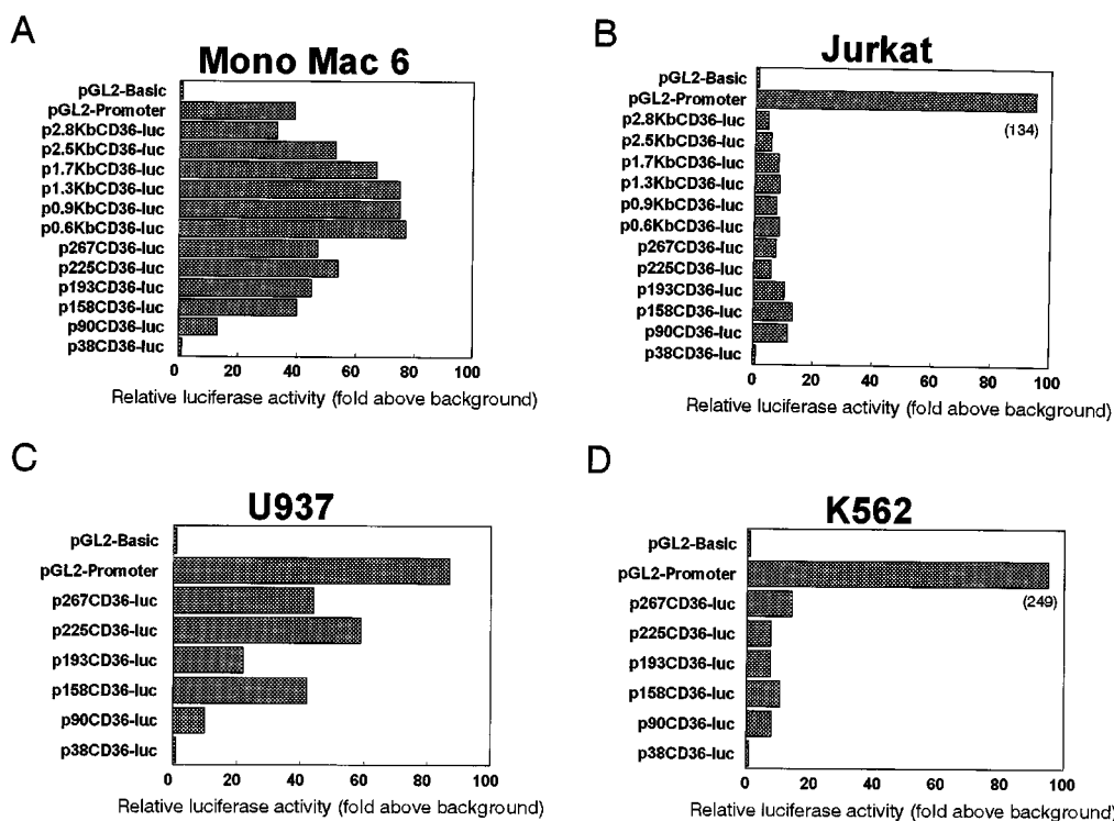
FIG. 1. Deletion analysis of CD36 promoter. A panel of CD36 promoter deletion constructs coupled to the reported luciferase gene were transiently transfected into the cell lines Mono Mac 6, U937, Jurkat, and K562, as described under "Experimental Procedures." Promoter activity of each construct was expressed as -fold activity above the background activity conferred by the promoterless control plasmid pGL2-Basic, corrected for transfection efficiency (Böttinger et al. , 1994). Number enclosed in parenthesis in charts B and D denote the relative luciferase activities yielded by the pGL2-promoter construct (which contains the SV40 promoter).
