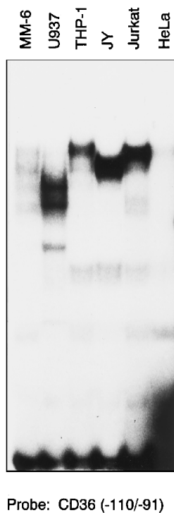
FIG. 3. Binding of CD36 promoter region -110/-91 to nuclear extracts from several cell lines. Radiolabeled double-stranded CD36 promoter -110/-91 oligonucleotide, GCAACAAACCACACTGGG, was incubated with nuclear extracts from cell lines of different origin (Mono Mac 6, U937, and THP-1, monocytic; JY, B lymphoblastoid; Jurkat, T cell leukemia; HeLa, epitheloid carcinoma).
