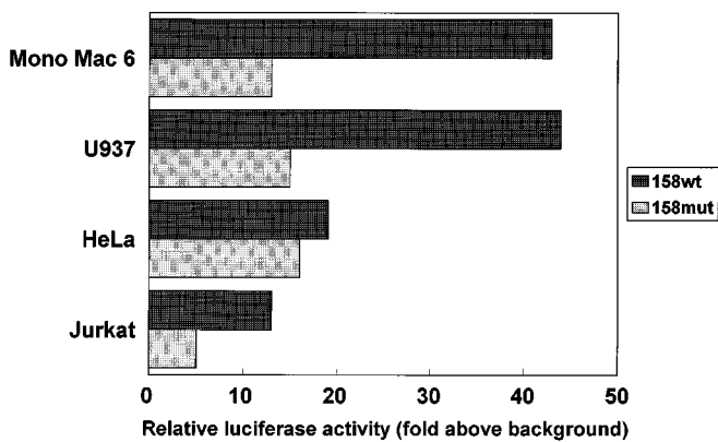
FIG. 2. Mutation of site -102/-98 severely impairs the activity of the CD36 promoter. CD36 promoter wild type construct pCD36-158-luc (represented as 158wt ) and mutant construct pCD36-158(m-102/-98)-luc (represented as 158mut ) were transiently transfected in Mono Mac 6, U937, Jurkat, and HeLa cells. For each cell line assayed, promoter activities were represented as indicated for Fig. 1.
